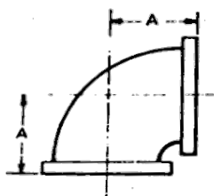
90° Female No. 151
