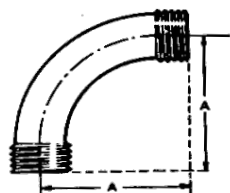
Male No. 191
